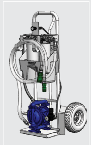
Basic - pneumatic
